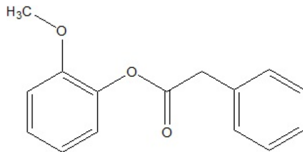
Guaiacyl Phenylacetate
